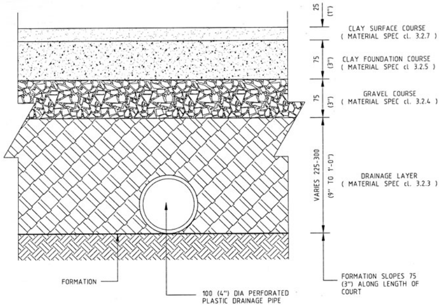
TYPICAL SECTION THROUGH COURT CONSTRUCTION LAYERS
