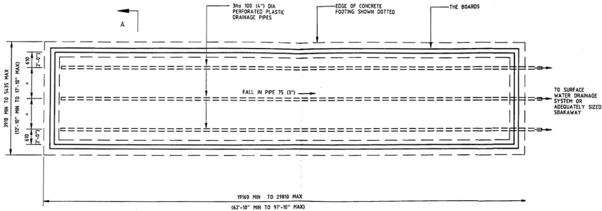
PLAN OF COURT
